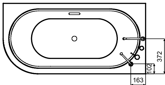
schemat 6/A
